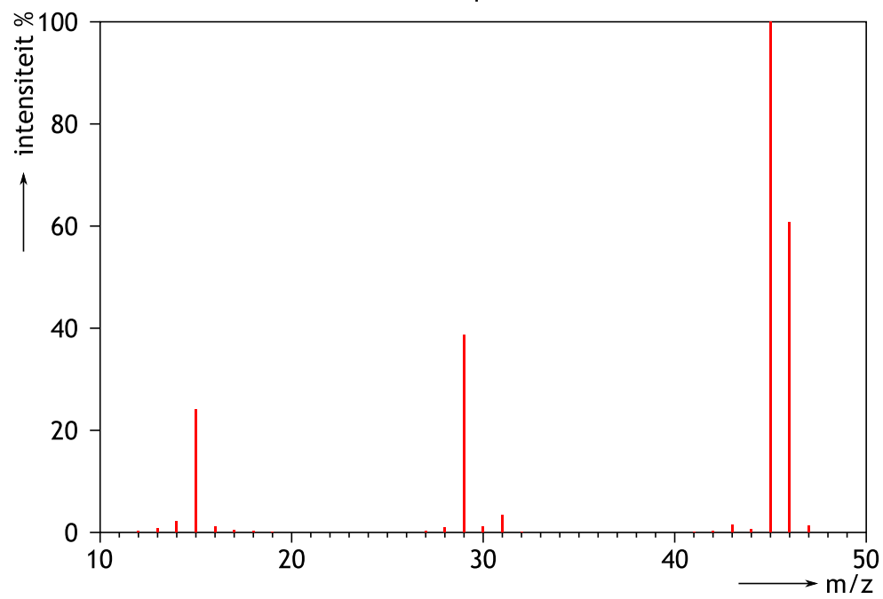
Massaspectrum
