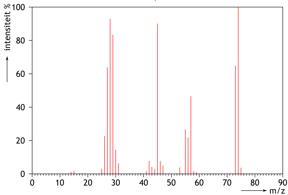
Massaspectrum
