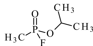
Sarin ( \text{C}_4\text{H}_{10}\text{FO}_2\text{P} )
