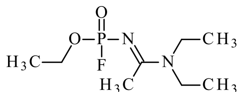
Novichok A-234
